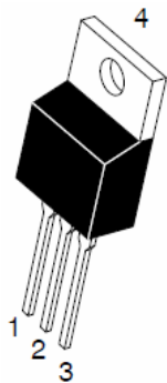
MUR2030CT TO-220AB
