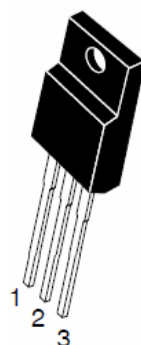
MUR2030CTF TO-220F
