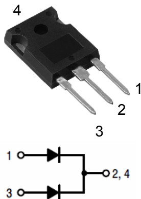
TO-247 MUR8060PT
