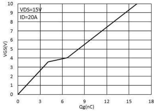
Figure 7: Gate-Charge Characteristics
