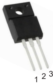
TO-220F MUR1660CTF-A
