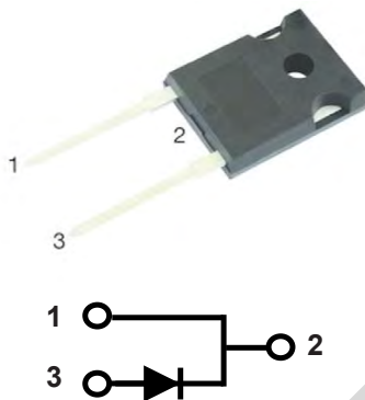
TO-247AC MURE6040APT
