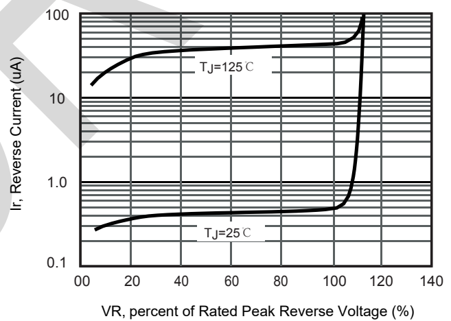
FIG.4-Typical Reverse Current
