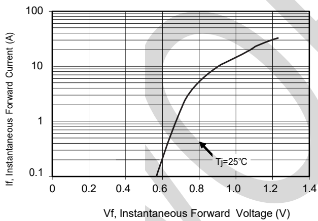
FIG.3-Typical Forward Voltage
