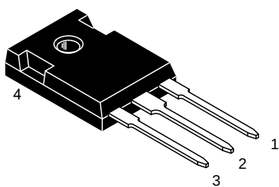
TO-247S TSR30V300PTS
