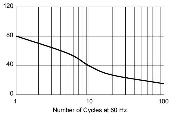
Maximum Repetitive Surge Current
