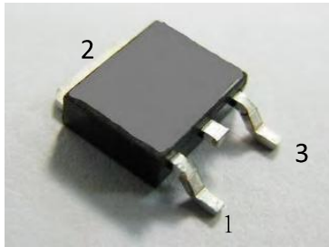
TSP20L45D TO-252
